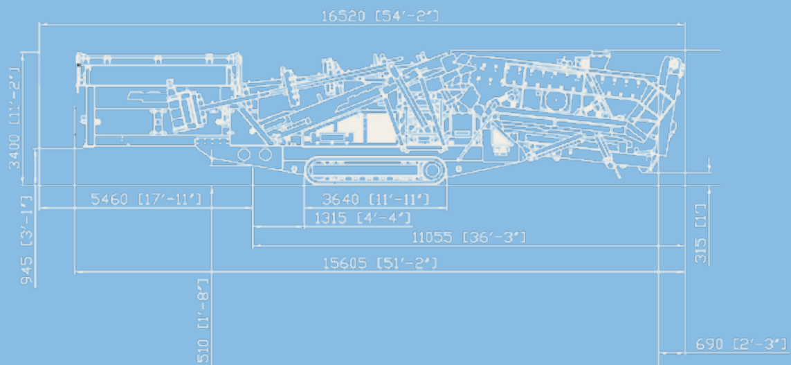
Side view MS 16 D transport position
